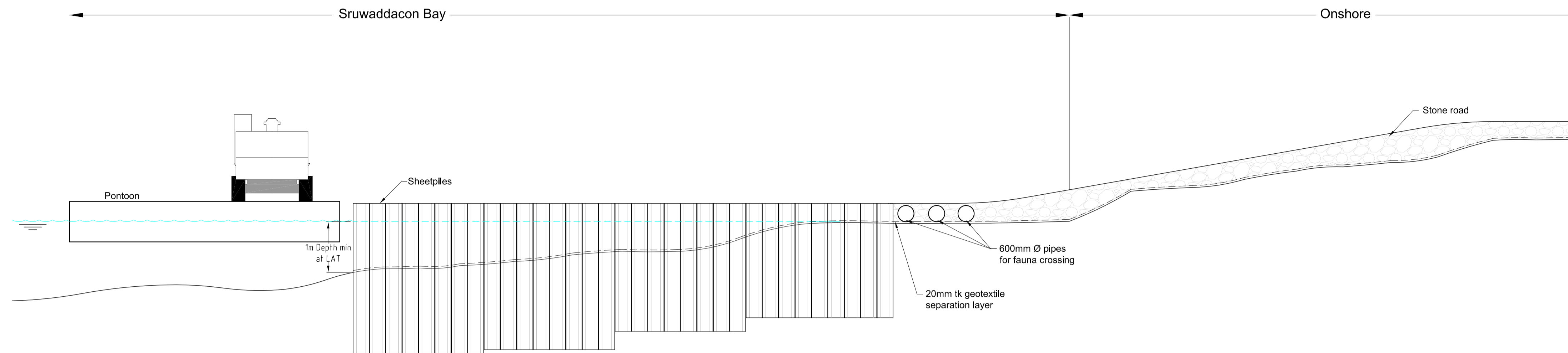
TYPICAL TEMPORARY SHORE ACCESS DETAIL - SECTION
