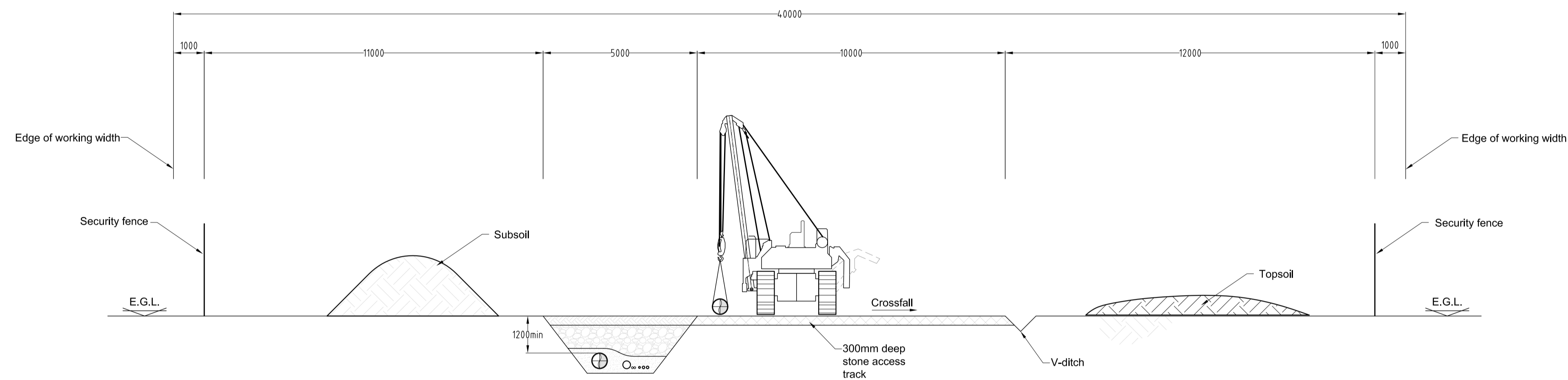
TYPICAL WORKING WIDTH CROSS SECTION SCALE 1:100 @ A1
