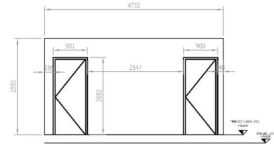
NORTH WESTERN ELEVATION
