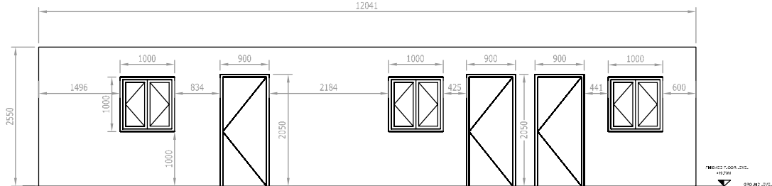
SOUTH EASTERN ELEVATION
