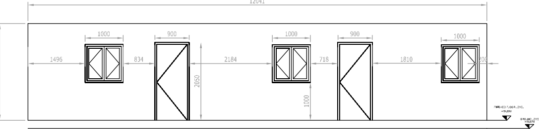
NORTHWEST ELEVATION
