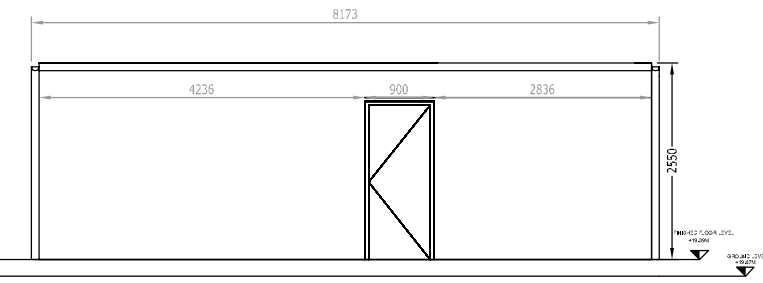
SOUTHEAST ELEVATION
