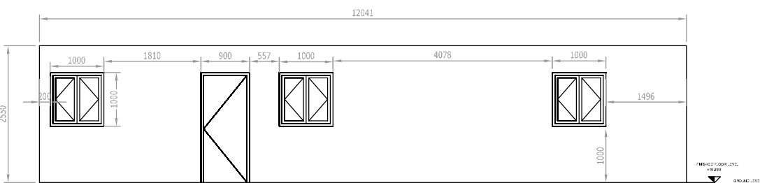
SOUTHEAST ELEVATION
