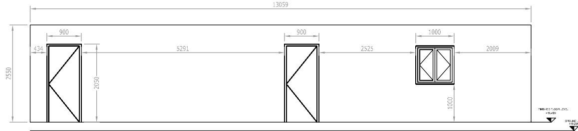
NORTHWEST ELEVATION
