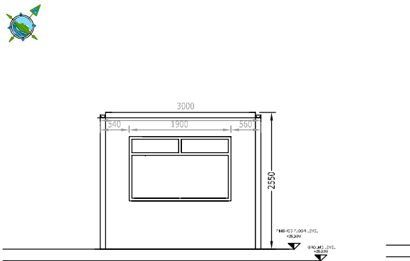
SOUTHWEST ELEVATION
