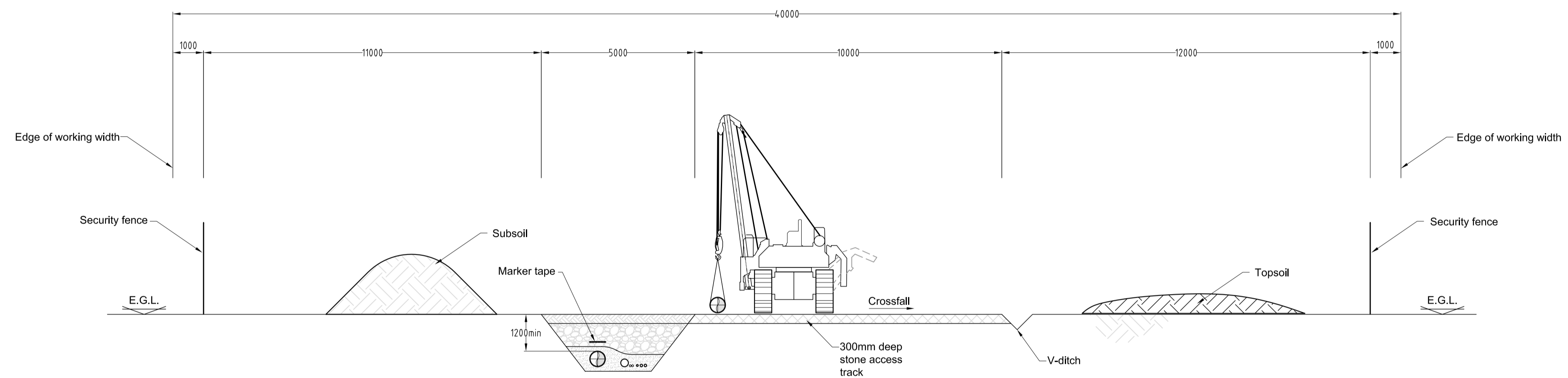
TYPICAL WORKING WIDTH CROSS SECTION SCALE 1:100 @ A1
